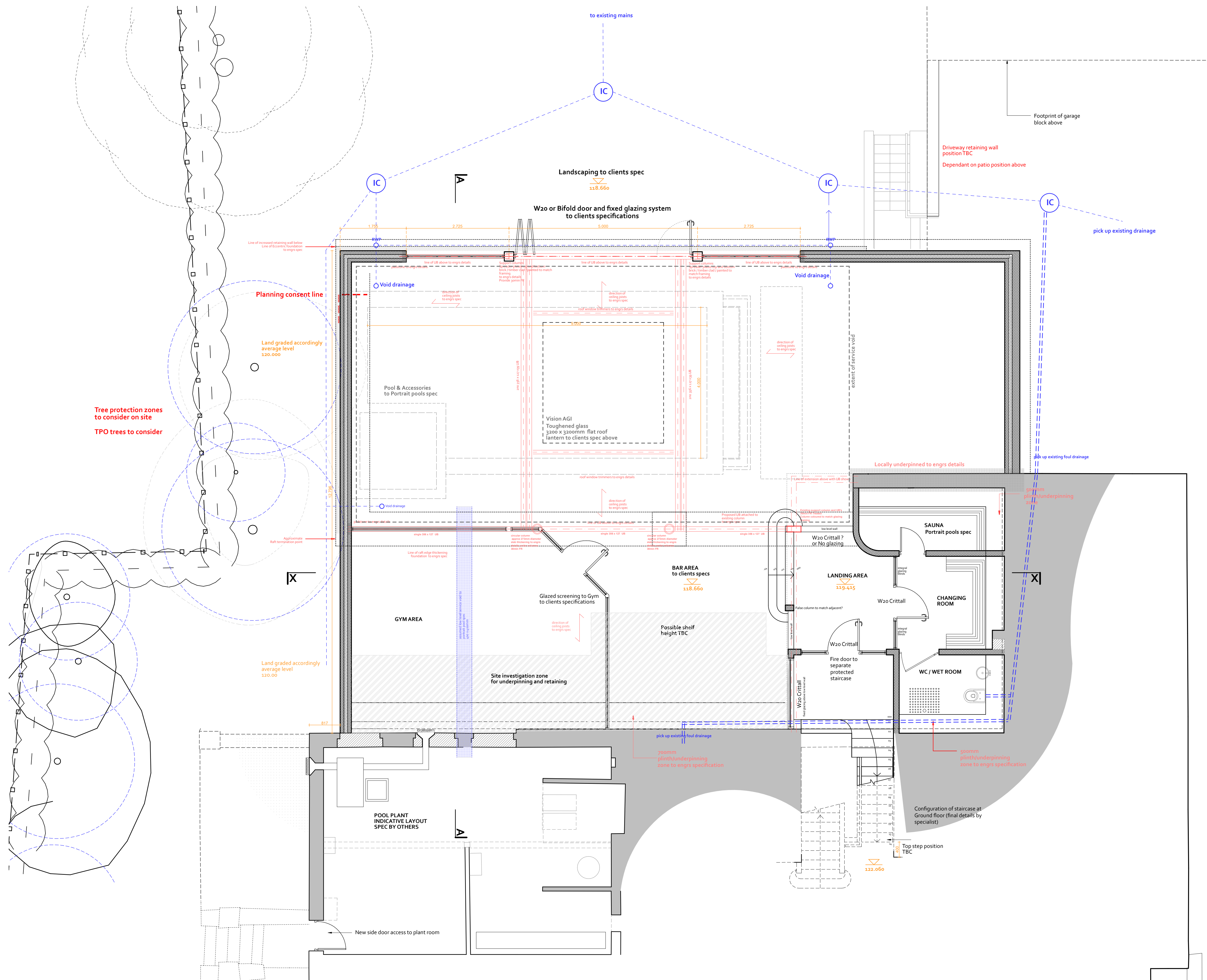
Proposed lower ground floor plan Draft issue only 24.02.22 Awaiting engrs input
